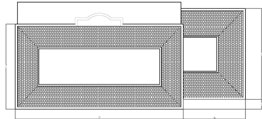
ROOF PLAN
